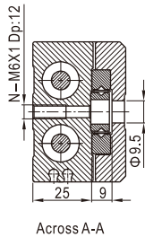
Across A-A
